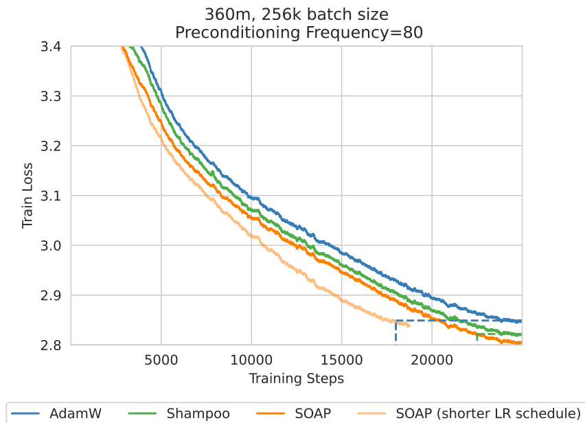
Figure 4: Comparing performance of tuned runs for AdamW, Shampoo (using DistributedShampoo (Shi et al., 2023) implementation) and SOAP for token batch size of 256k. Shampoo and SOAP use preconditioning frequency of 80. We observe a \geq 25\% reduction in the number of iterations compared to AdamW, and approximately a 10% reduction compared to Shampoo. See Figure 2 (right) for wall-clock time improvement and Section 5 for detailed calculation of efficiency improvement.
